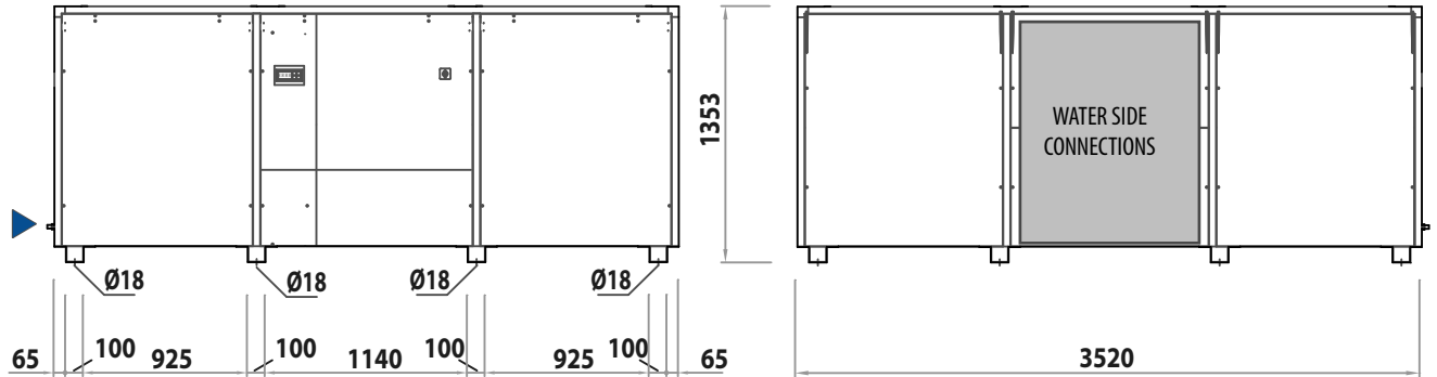
FRONT VIEW
